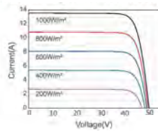
Current-Voltage Curve GSE HC 540 - 144M
