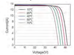
Current-Voltage Curve GSE HC 540 - 144M
