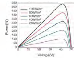
Power-Voltage Curve GSE HC 540 - 144M
